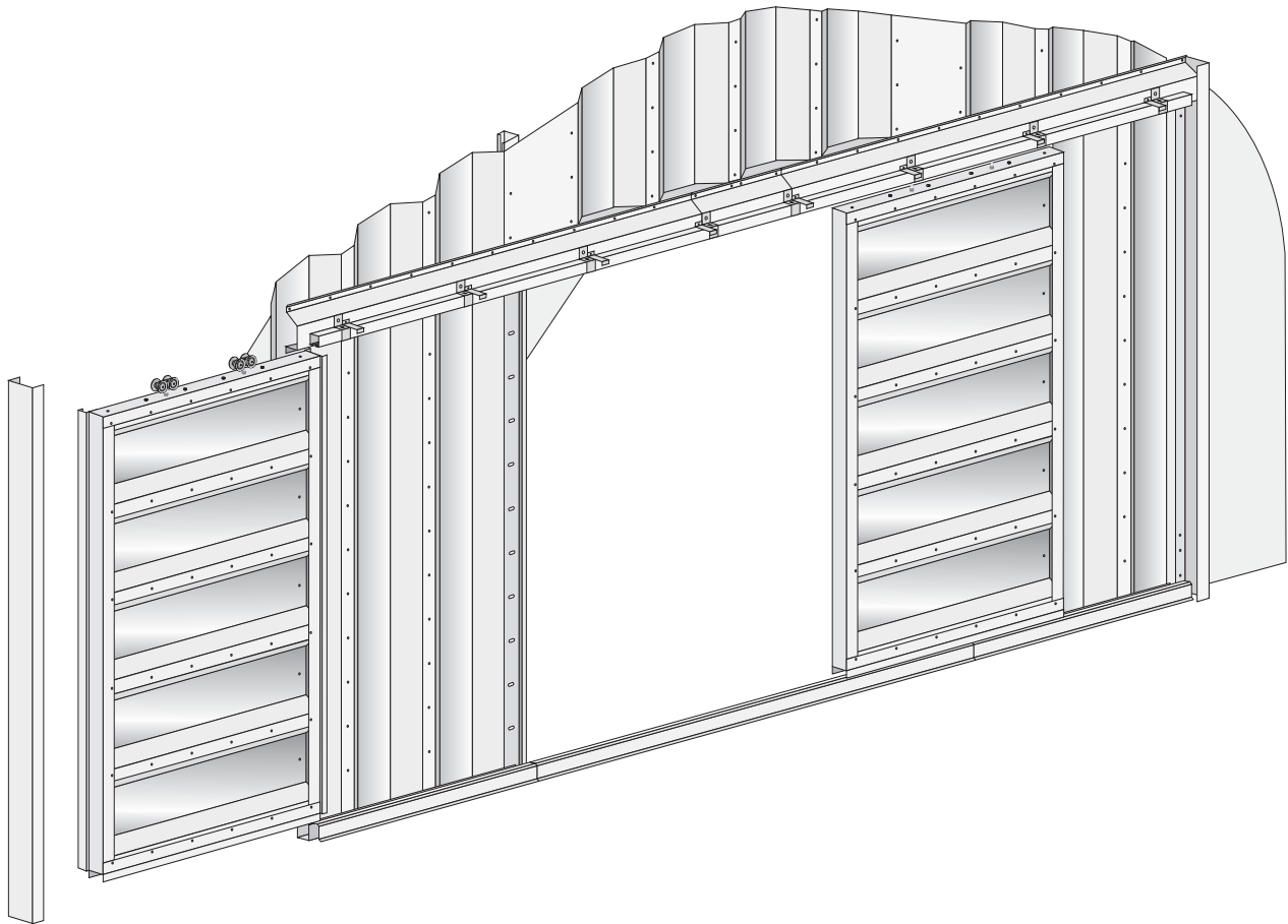
FIGURE 71: INSTALLING THE SLIDING DOOR
