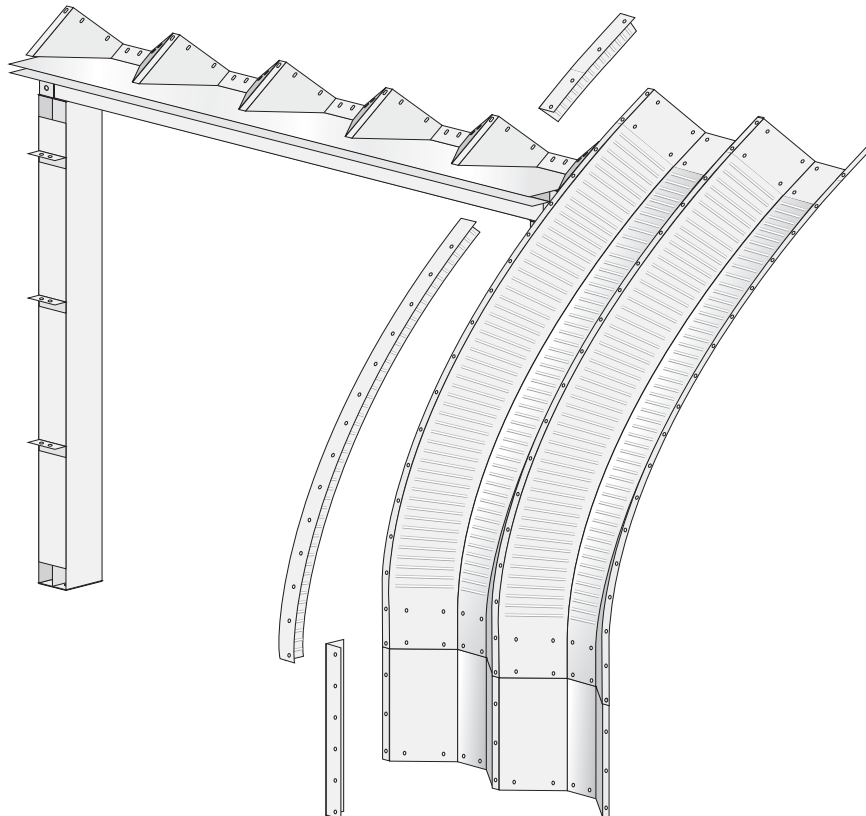
FIGURE 36: INTERIOR FRAME FOR SIDE OPENING WITH CANOPY
