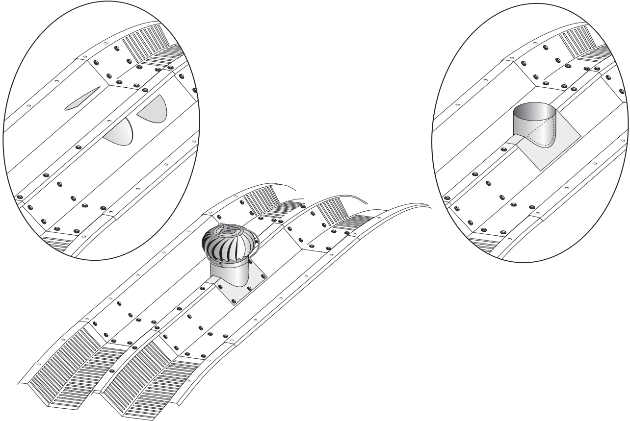
FIGURE 75: VENTILATOR ADAPTORS & TURBINE VENTS
