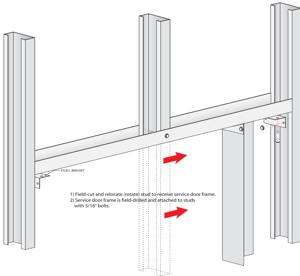
FIGURE 56: ADJUSTING STUDS FOR SERVICE DOORS/WINDOW FRAMES
