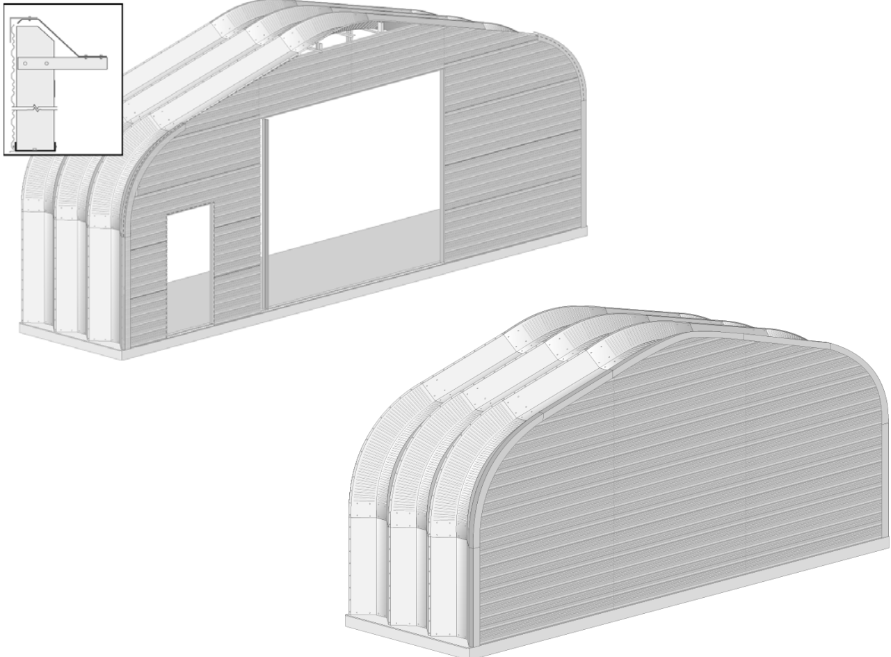
FIGURE 59: INSTALLING SHEETING
