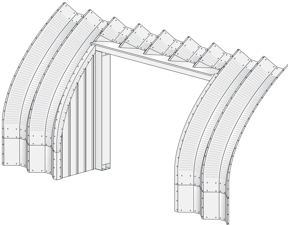
FIGURE 34: COMPLETE RECESSED SIDE OPENING
