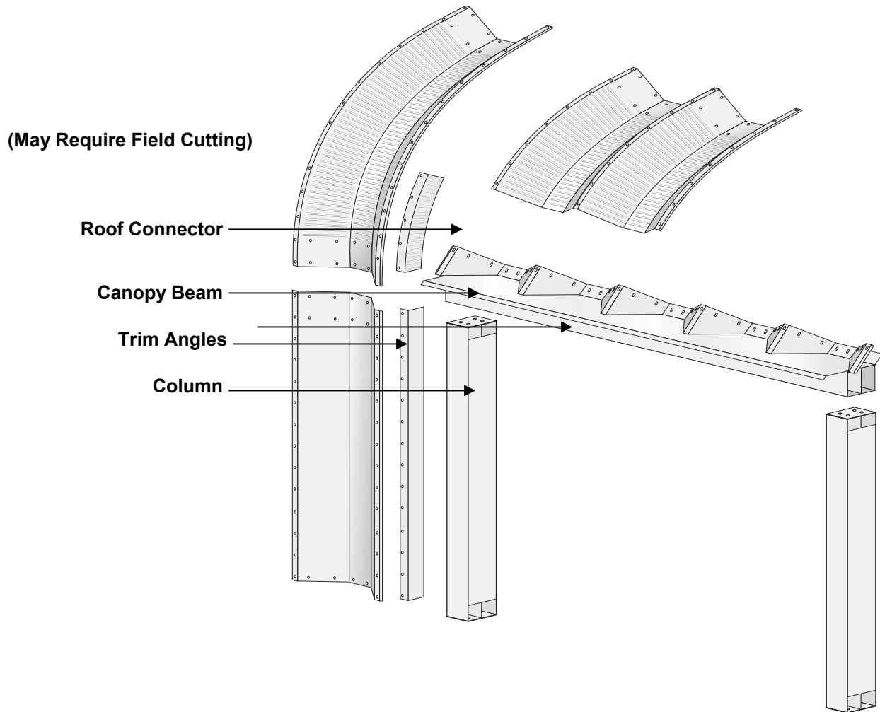
FIGURE 32: SIDE OPENING WITHIN STRAIGHT WALL
