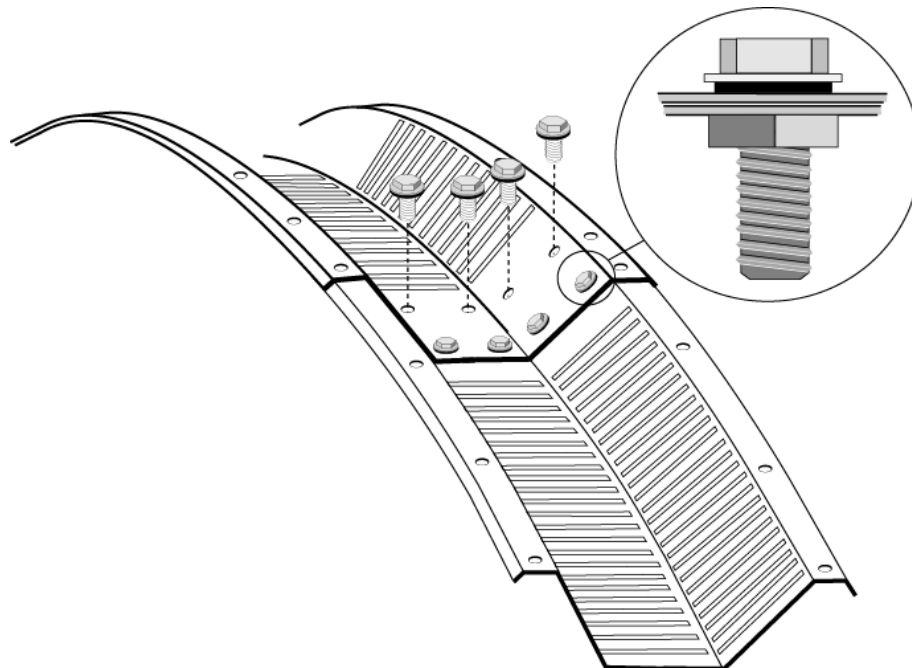
FIGURE 20: CONNECTING PANELS
