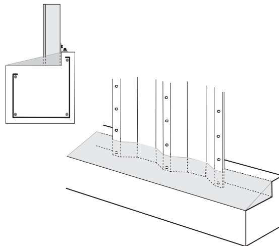
FIGURE 85: GROUTING THE END WALLS
