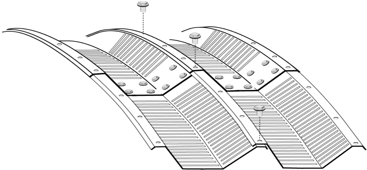
FIGURE 27: CONNECTING ARCH TO ARCH DURING CONSTRUCTION
