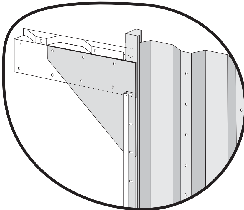
FIGURE 62: ATTACHMENT PLATES
