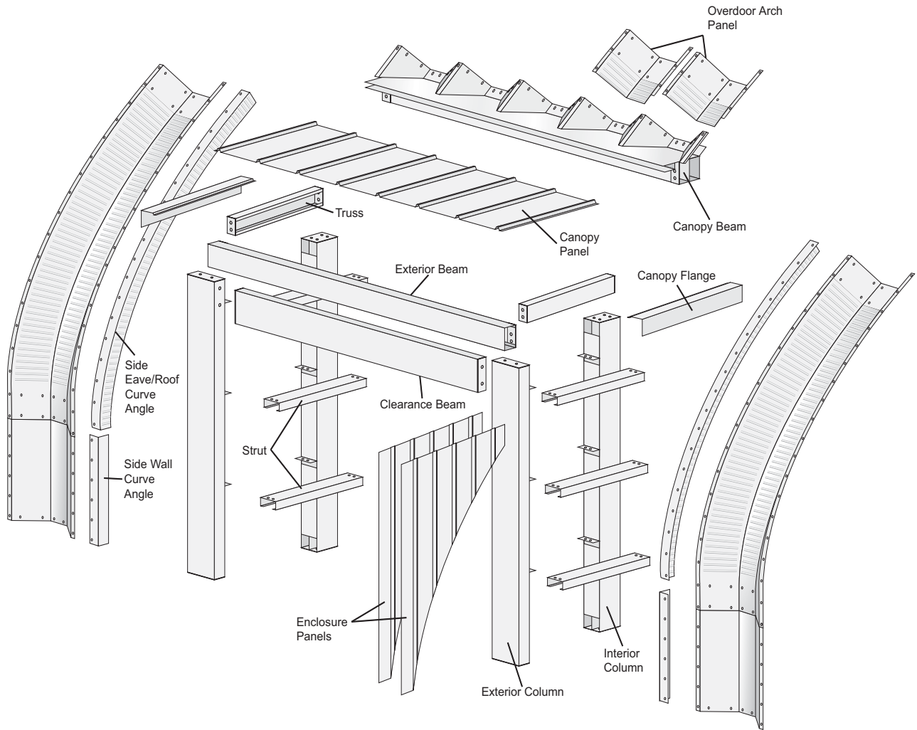
FIGURE 36: INTERIOR FRAME FOR SIDE OPENING WITH CANOPY
