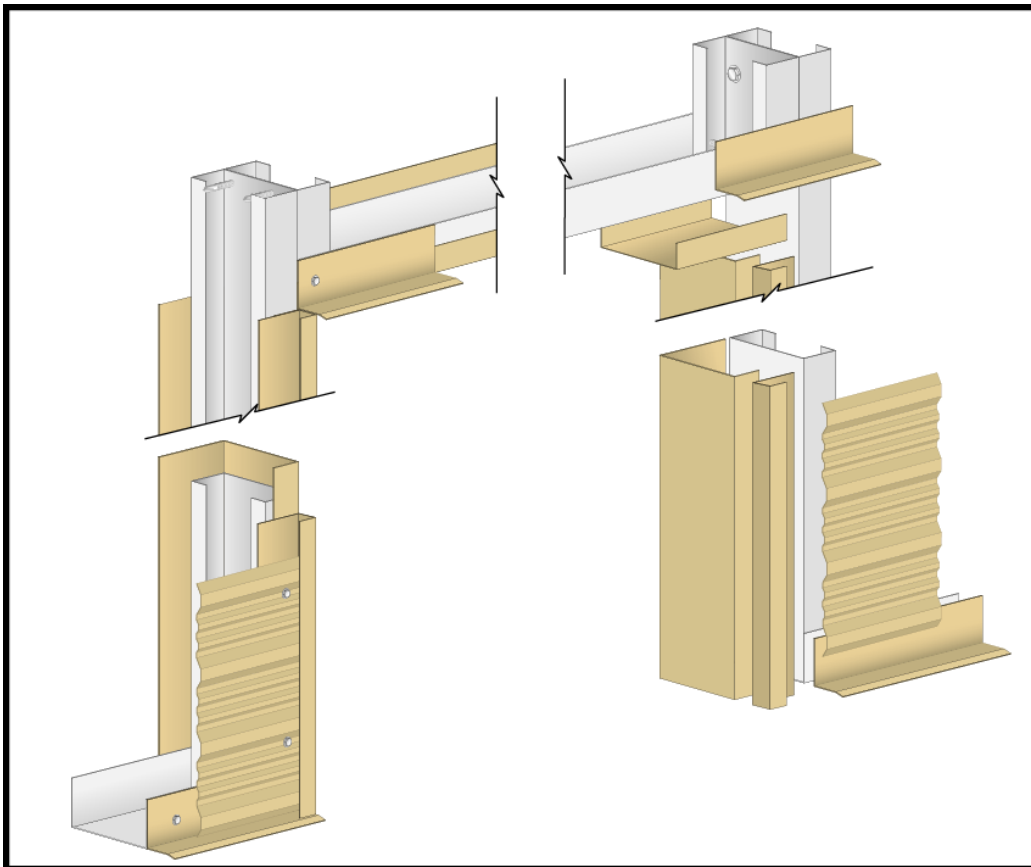
FIGURE 55: FLASHING FOR OVERHEAD DOOR IN CLADDED END WALL
