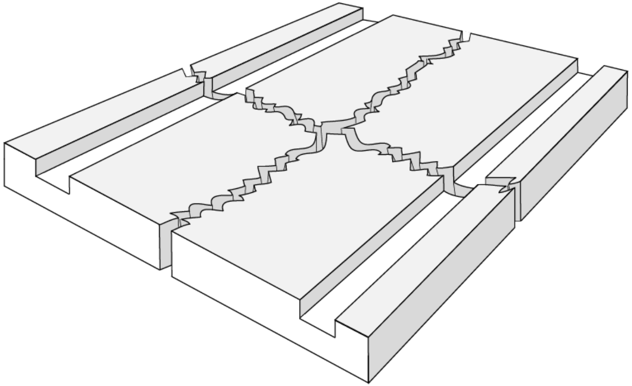
FIGURE 2: STANDARD FOUNDATION (WITHOUT END WALLS)
