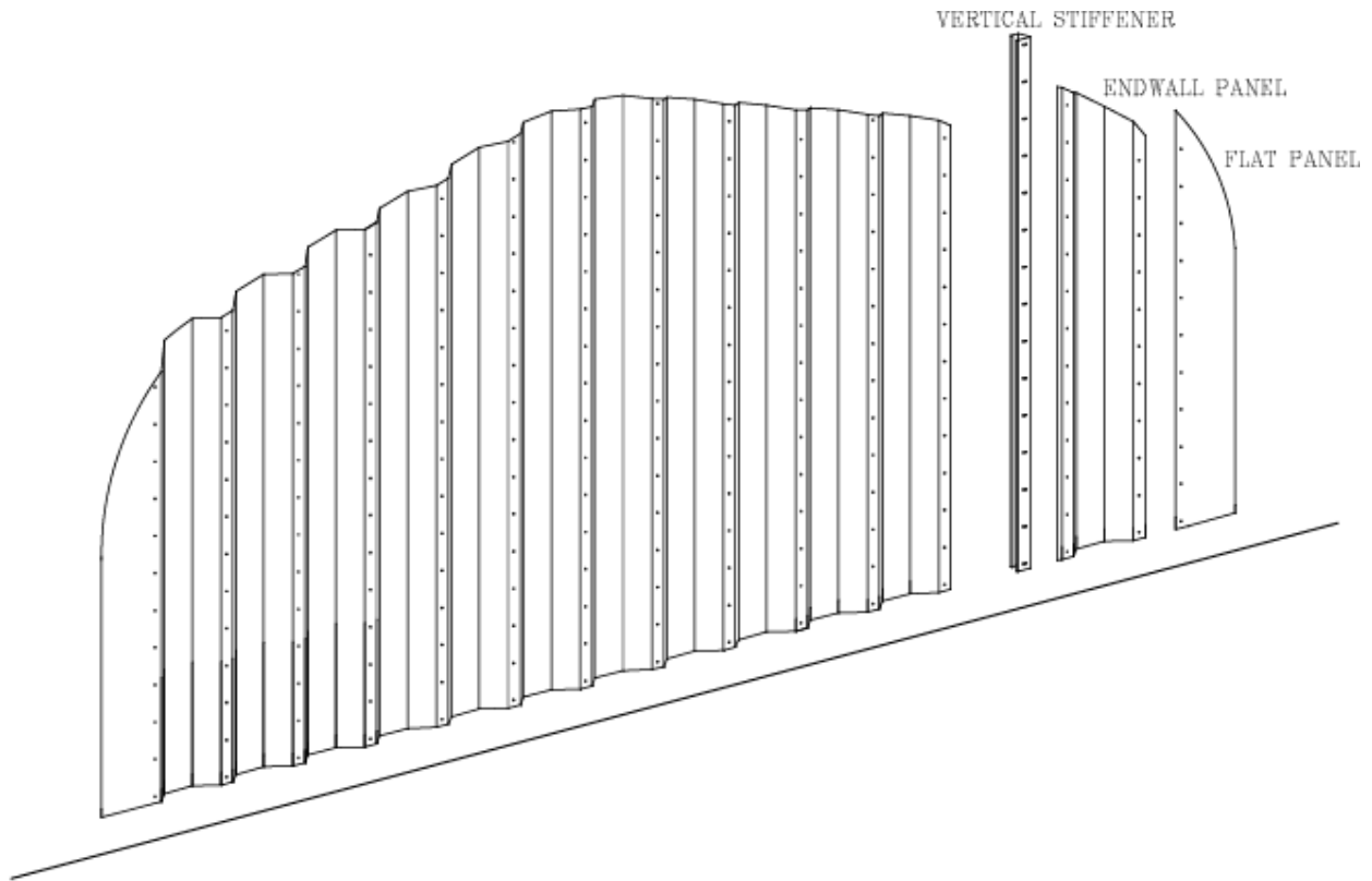
FIGURE 88: INSTALLING VERTICAL STIFFENERS
