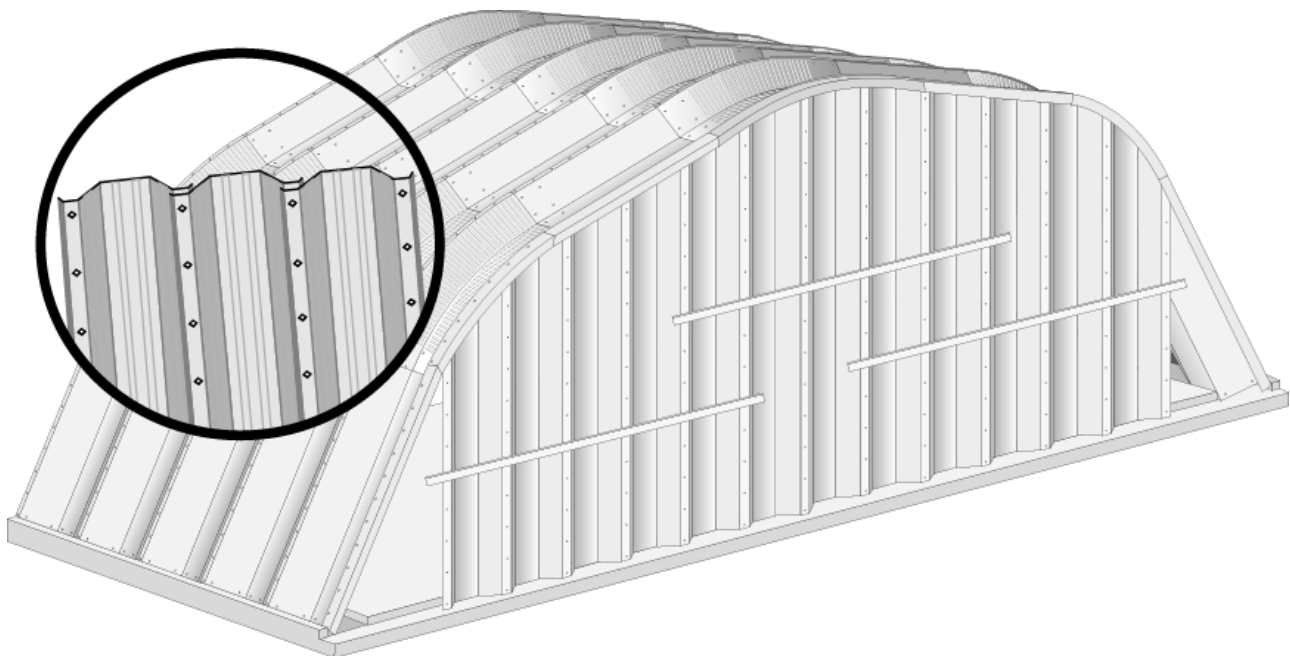
FIGURE 43: USING END WALL STRAPPING FOR CORRUGATED PANELS
