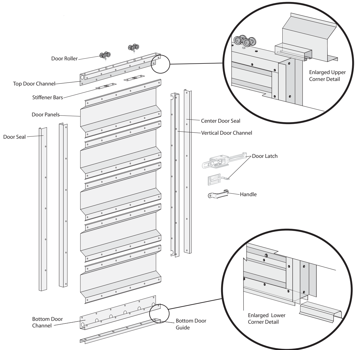
FIGURE 68: EXPLODED VIEW OF SLIDING DOORS
