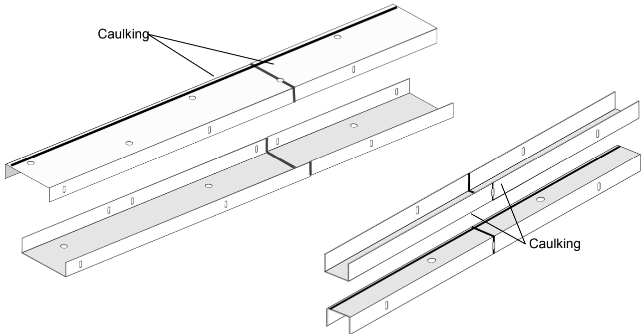
FIGURE 10: CAULKING C-CHANNEL CONNECTOR
