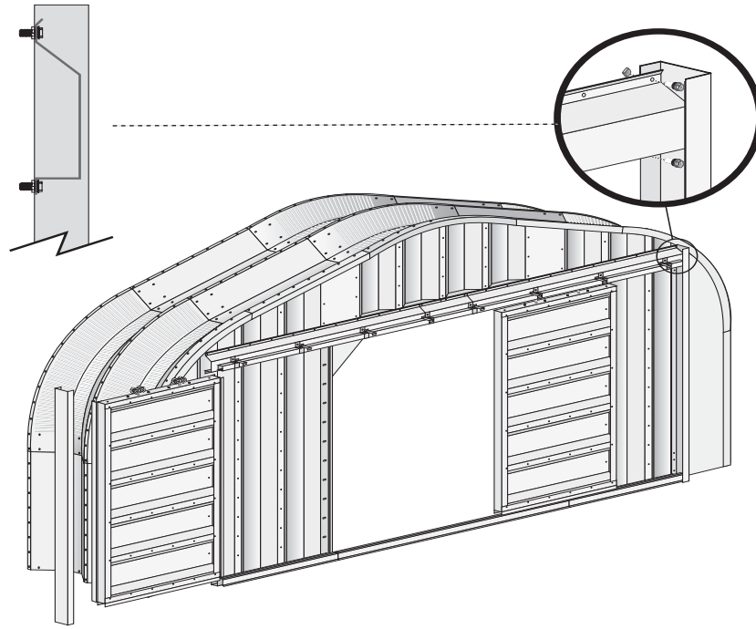
FIGURE 66: SLIDING DOOR WIND BRACING
