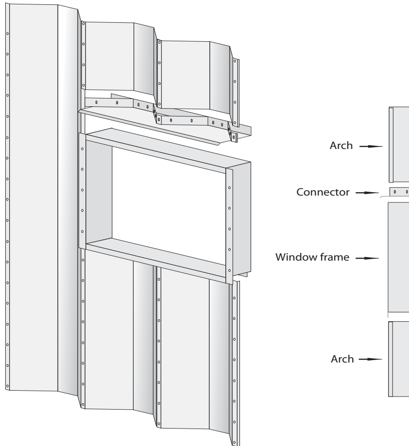
FIGURE 82: INSTALLING SIDE WINDOW FRAME
