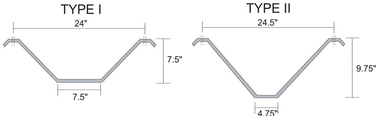
FIGURE 12: ARCH PANEL TYPES
