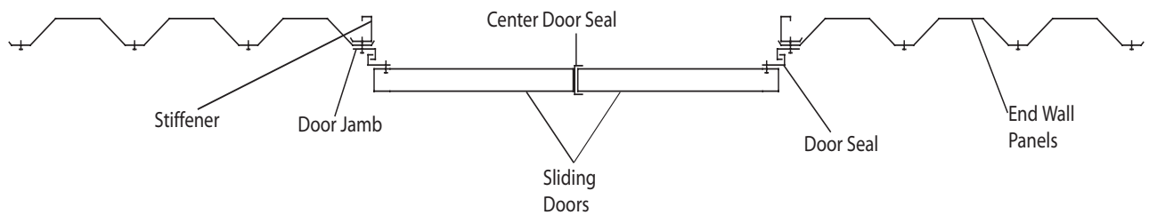
FIGURE 72: OVERHEAD VIEW OF COMPLETED ASSEMBLY
