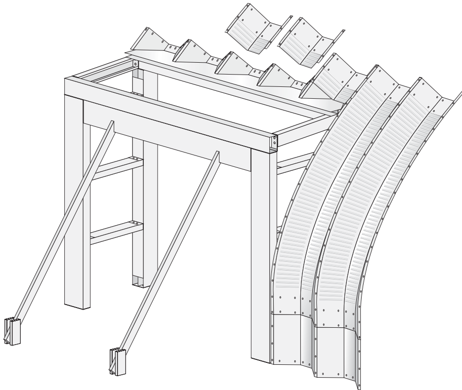
FIGURE 38: BRACING FRAMEWORK FOR SIDE OPENING WITH CANOPY
