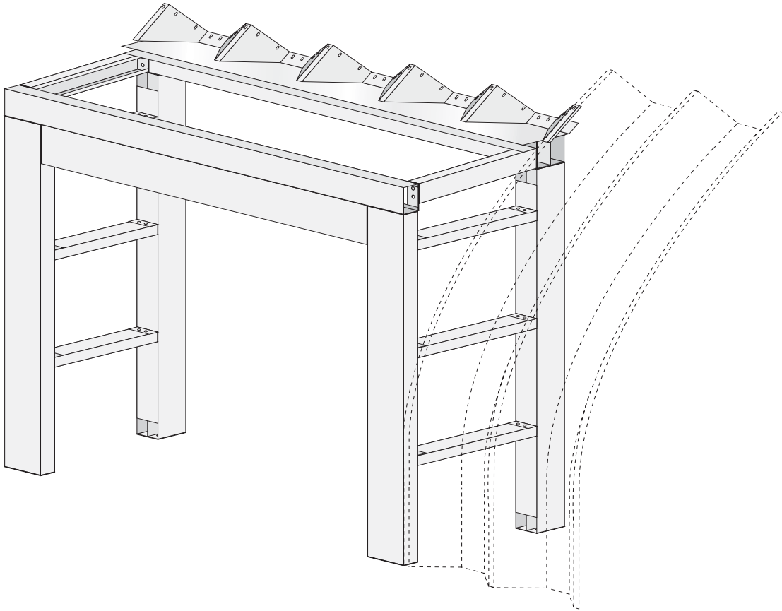
FIGURE 37: EXTERIOR FRAME & SUPPORT FOR SIDE OPENING WITH CANOPY
