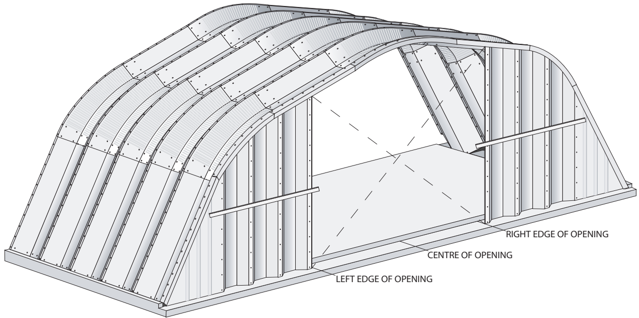
FIGURE 46: INSTALLING THE PANELS NEXT TO THE OPENING
