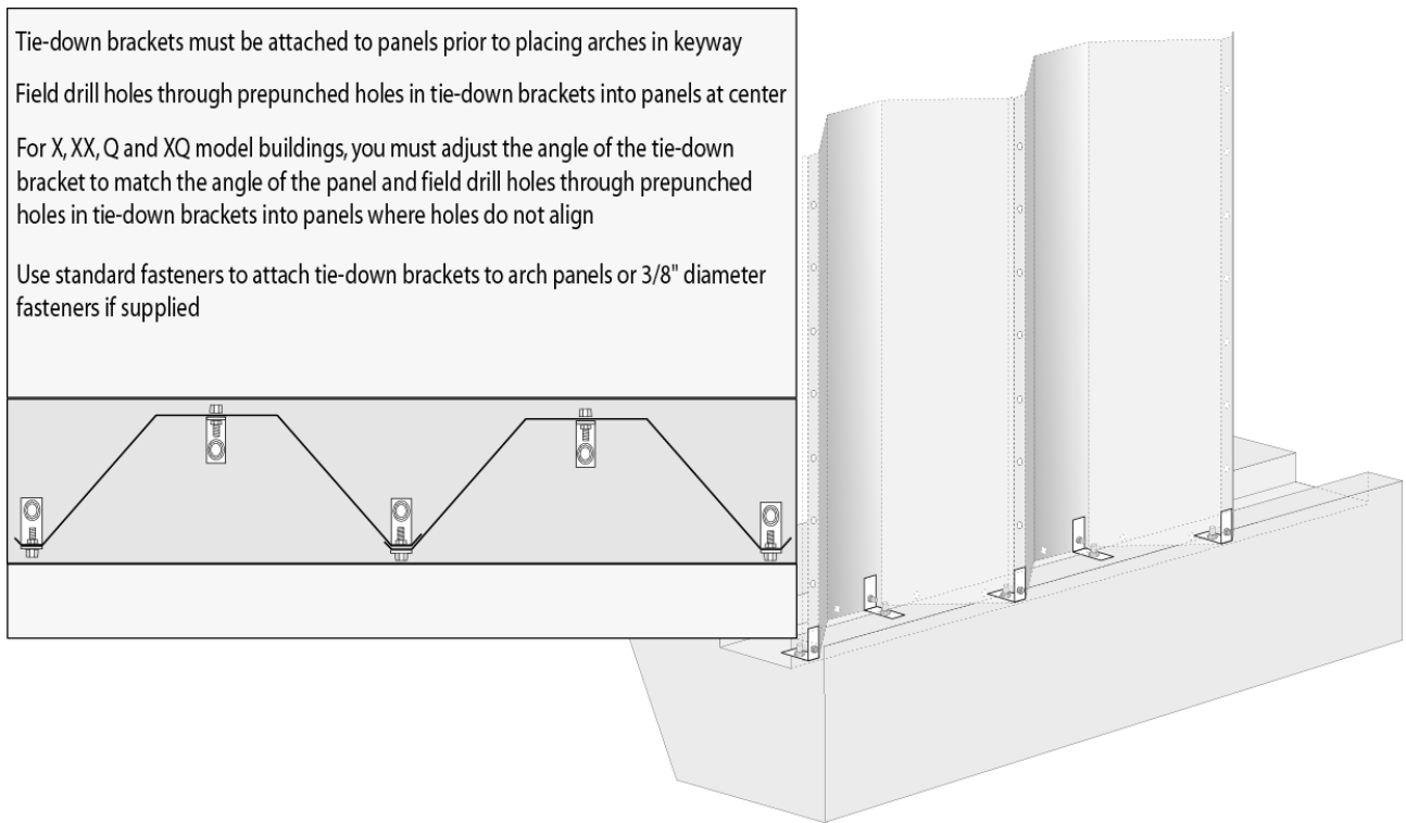
FIGURE 4: TYPICAL ANCHOR BOLTS AND TIE DOWN BRACKETS (ARCHES)
