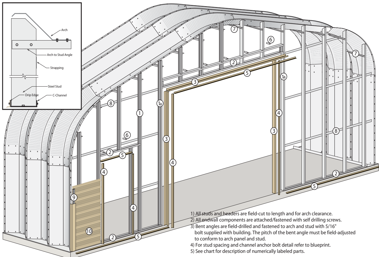
FIGURE 53: FRAMING THE CLADDED END WALL
