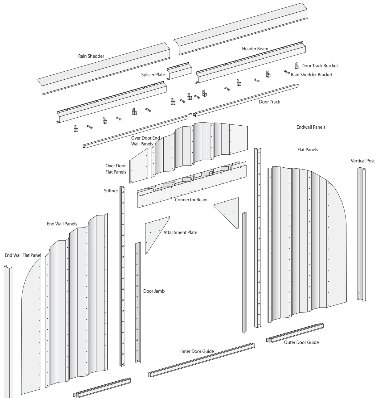
FIGURE 61: EXPLODED VIEW OF SLIDING DOOR FRAMING COMPONENTS
