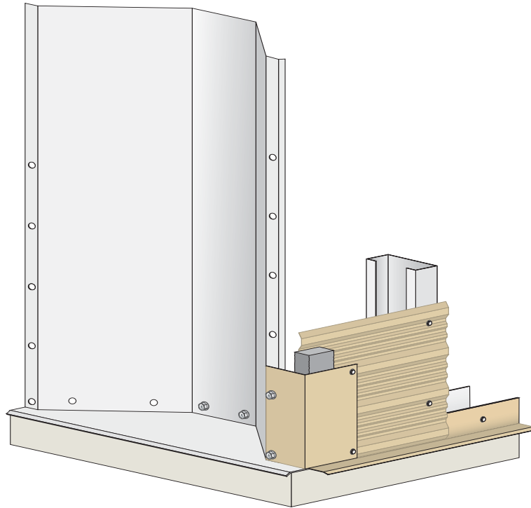
FIGURE 58: CLADDED END WALL CORNER DETAIL
