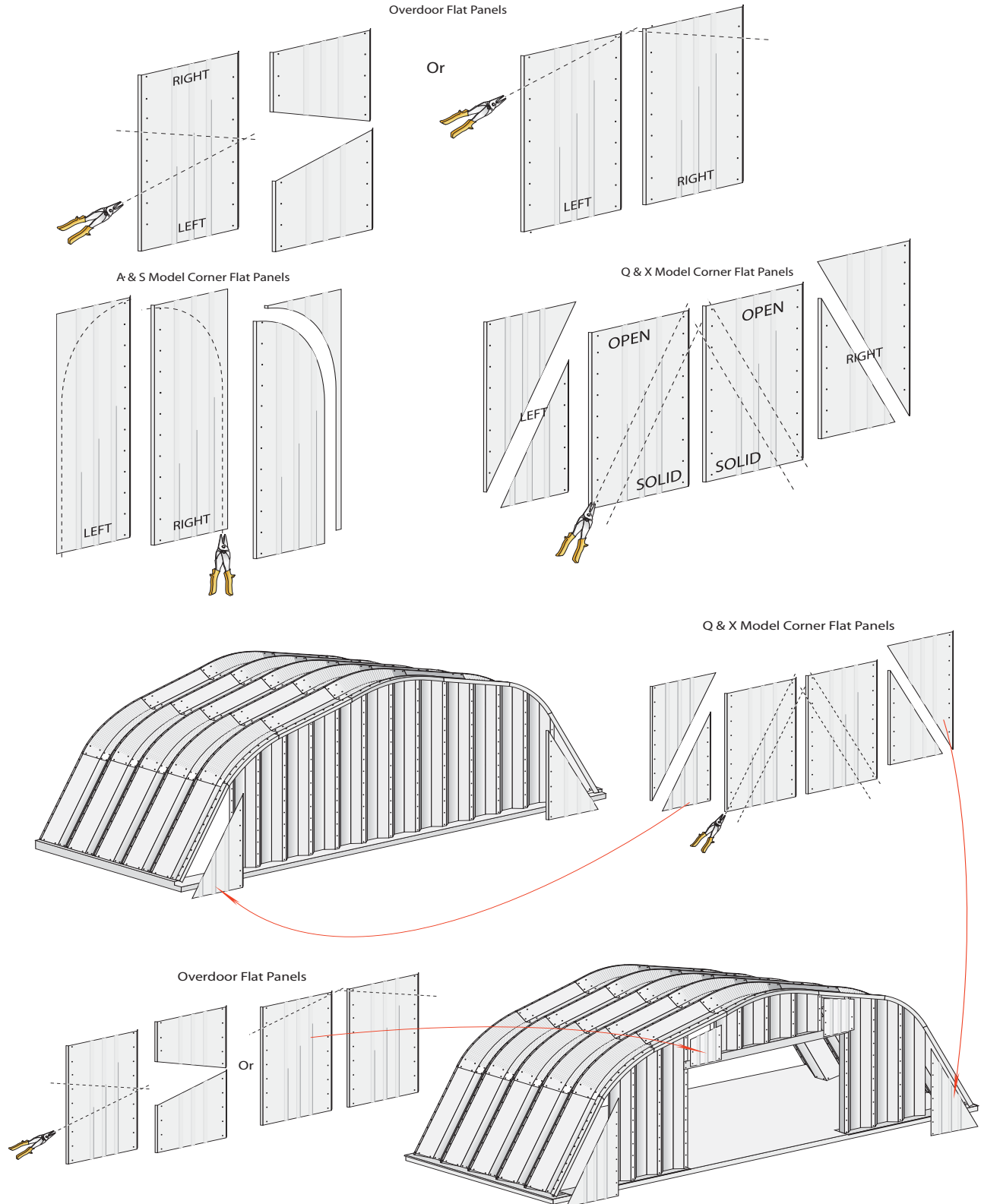
FIGURE 44: FIELD CUTTING THE CORNER PANELS & FLAT PANELS
