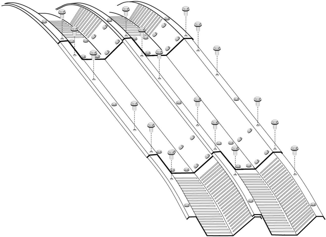
FIGURE 40: INSTALLING THE REMAINING BOLTS
