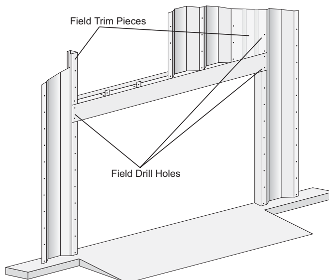
FIGURE 49: INSTALLING END WALL PANELS ABOVE DOOR FRAME
