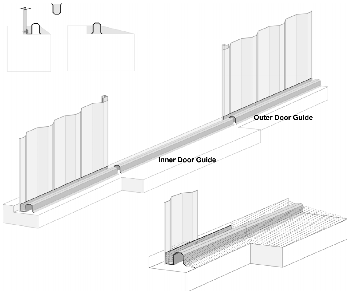
FIGURE 67: INNER AND OUTER DOOR GUIDES
