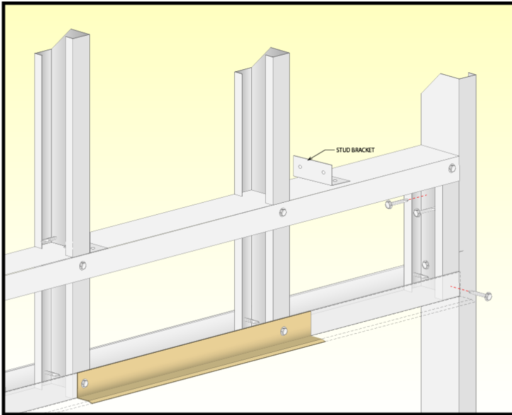
FIGURE 55: FLASHING FOR OVERHEAD DOOR IN CLADDED END WALL
