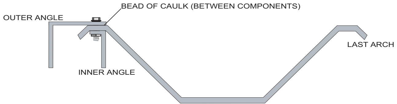
FIGURE 23: CROSS SECTION OF EXTENDED CURVE ANGLES
