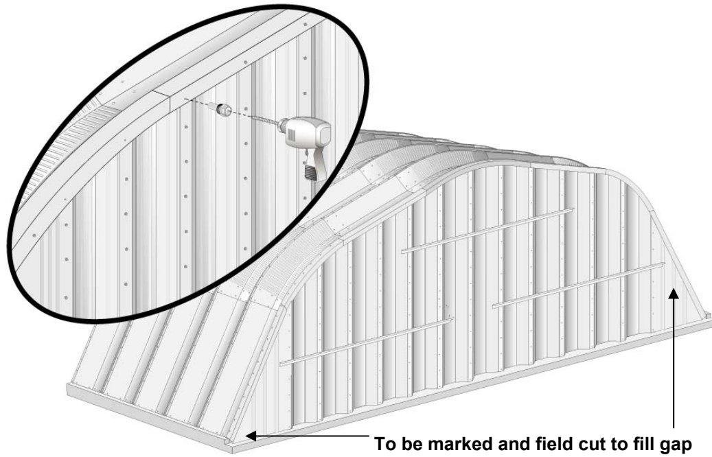
FIGURE 45: INSTALLING THE FLAT PANELS & SECURING THE END WALL
