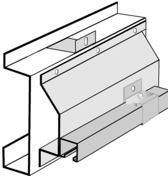
FIGURE 64: HEADER BEAM AND DOOR TRACK ASSEMBLY
