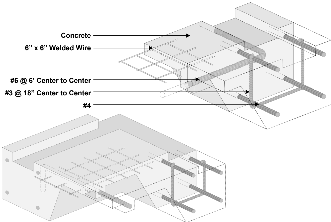
FIGURE 1: CROSS SECTIONS OF TYPICAL STANDARD FOUNDATION
