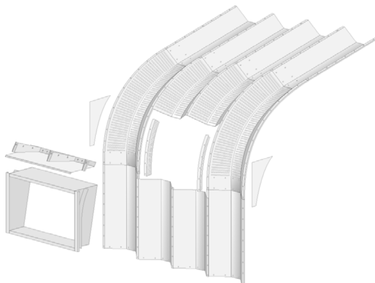
FIGURE 83: SIDE WINDOW FRAME WITH CANOPY FOR CURVED PANELS
