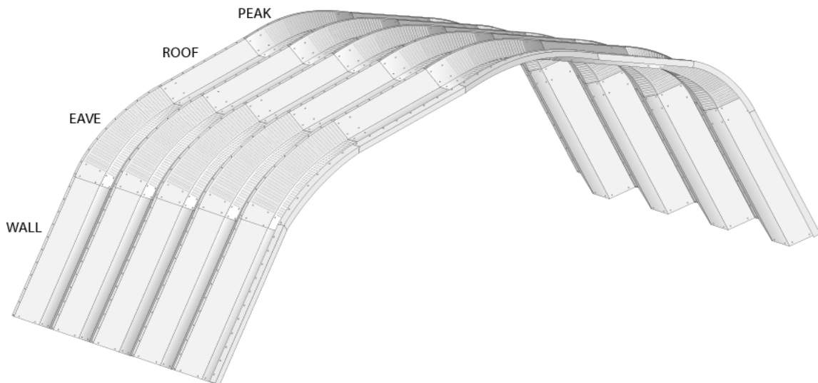
FIGURE 16: ANATOMY OF A TYPICAL X OR XX MODEL BUILDING
