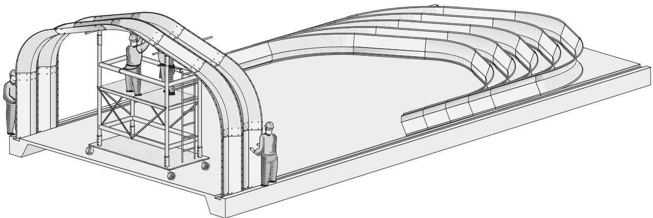
FIGURE 26: RAISING THE REMAINING ARCHES
