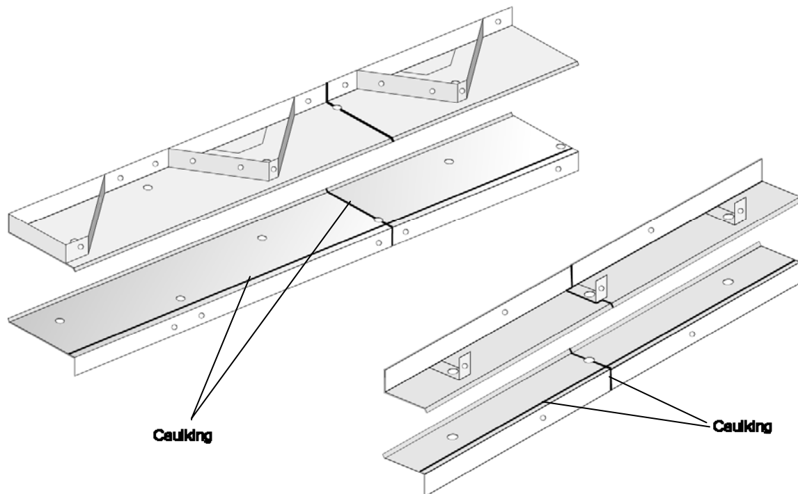
FIGURE 9: CAULKING INDUSTRIAL CONNECTOR
