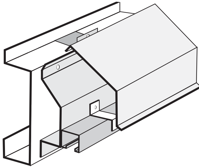
FIGURE 71: INSTALLING THE SLIDING DOOR
