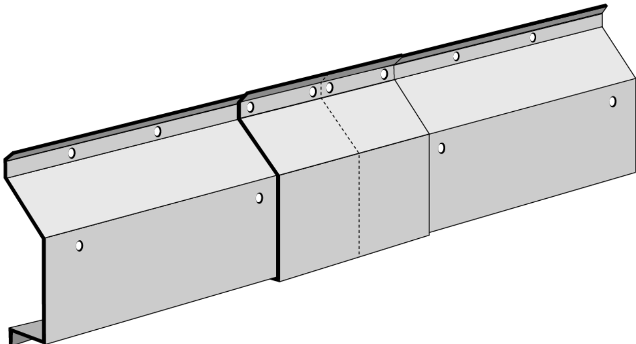
FIGURE 63: ASSEMBLING THE HEADER BEAM
