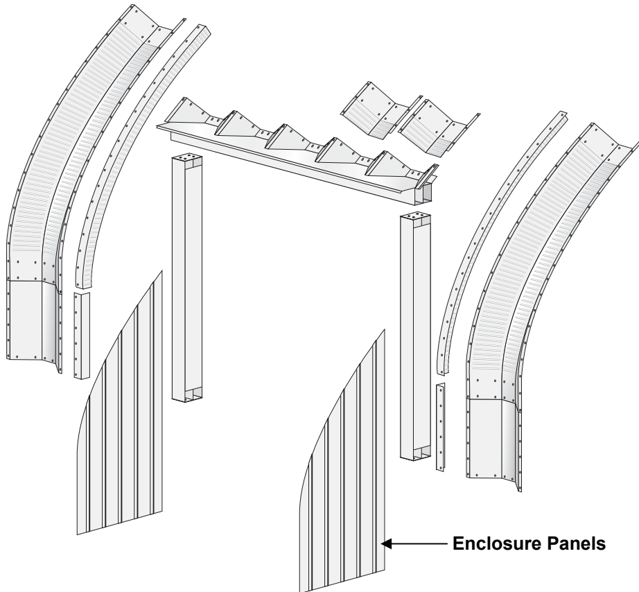
FIGURE 34: COMPLETE RECESSED SIDE OPENING
