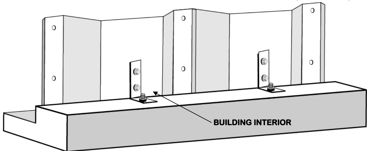
FIGURE 5: TYPICAL ANCHOR BOLTS AND TIE DOWN BRACKETS (END WALLS)
