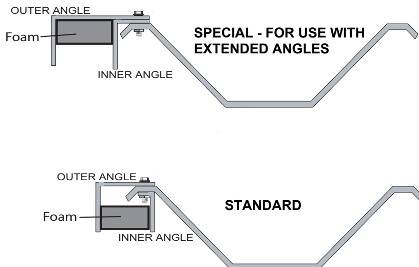
FIGURE 41: INSTALLING FOAM STRIPS
