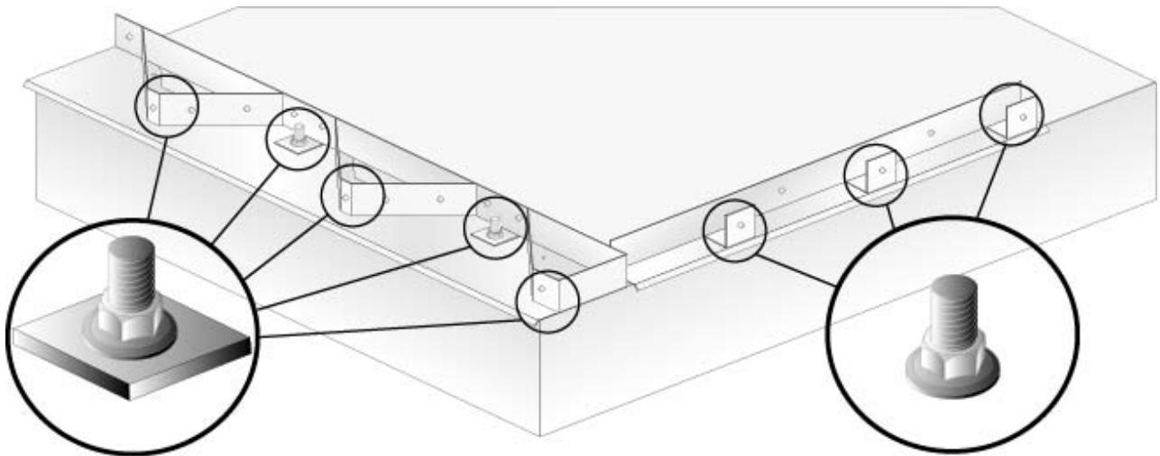
FIGURE 11: CORNER WITH INDUSTRIAL CONNECTORS
