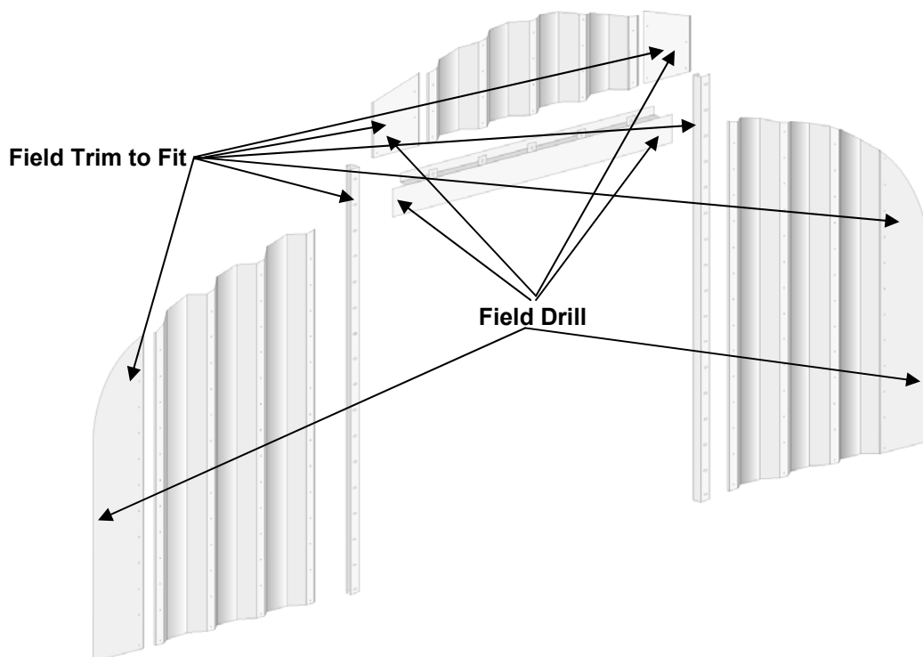
FIGURE 47: EXPLODED VIEW OF END WALL WITH FRAMED OPENING
