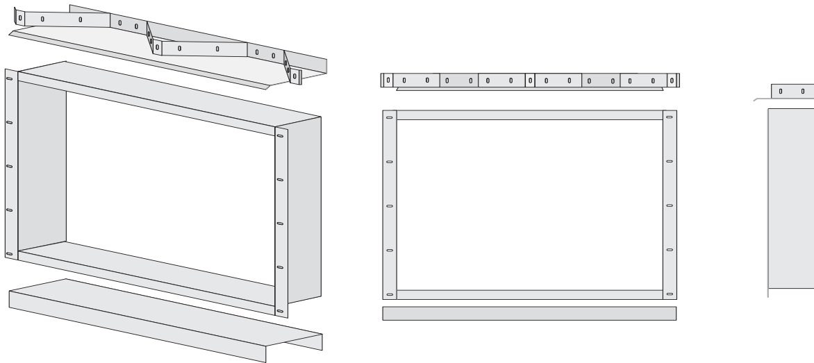
FIGURE 81: SIDE WINDOW FRAME (FOR STRAIGHT WALL ONLY)
