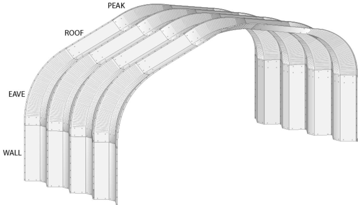
FIGURE 13: ANATOMY OF A TYPICAL A OR XA MODEL BUILDING
