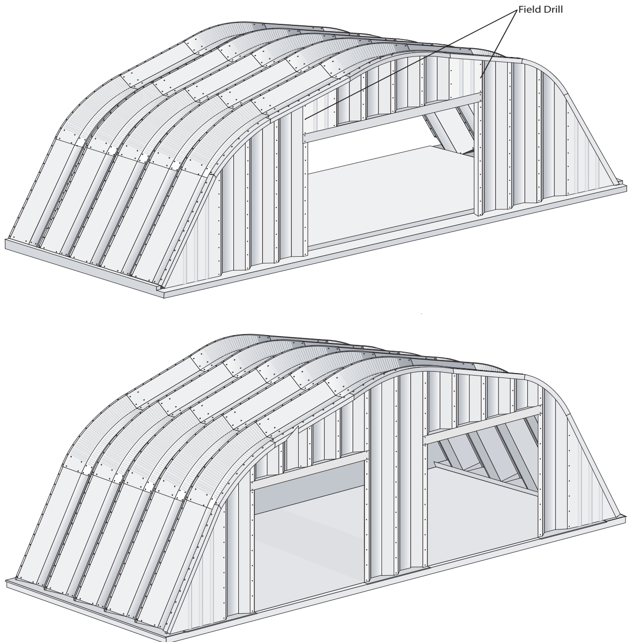
FIGURE 50: COMPLETE END WALLS WITH OPENINGS
