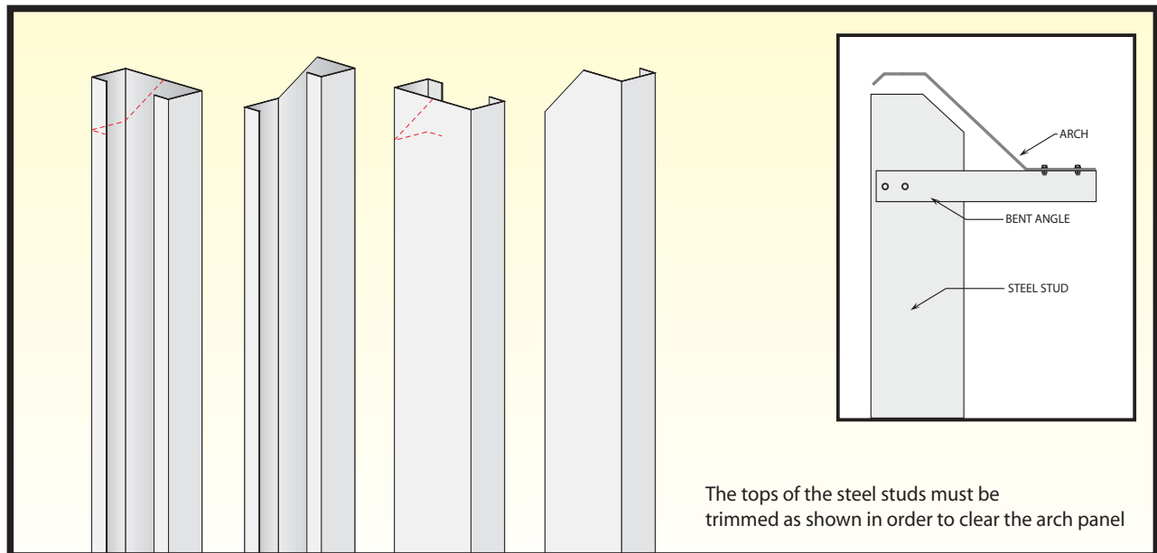
FIGURE 52: TRIMMING THE STEEL STUDS
