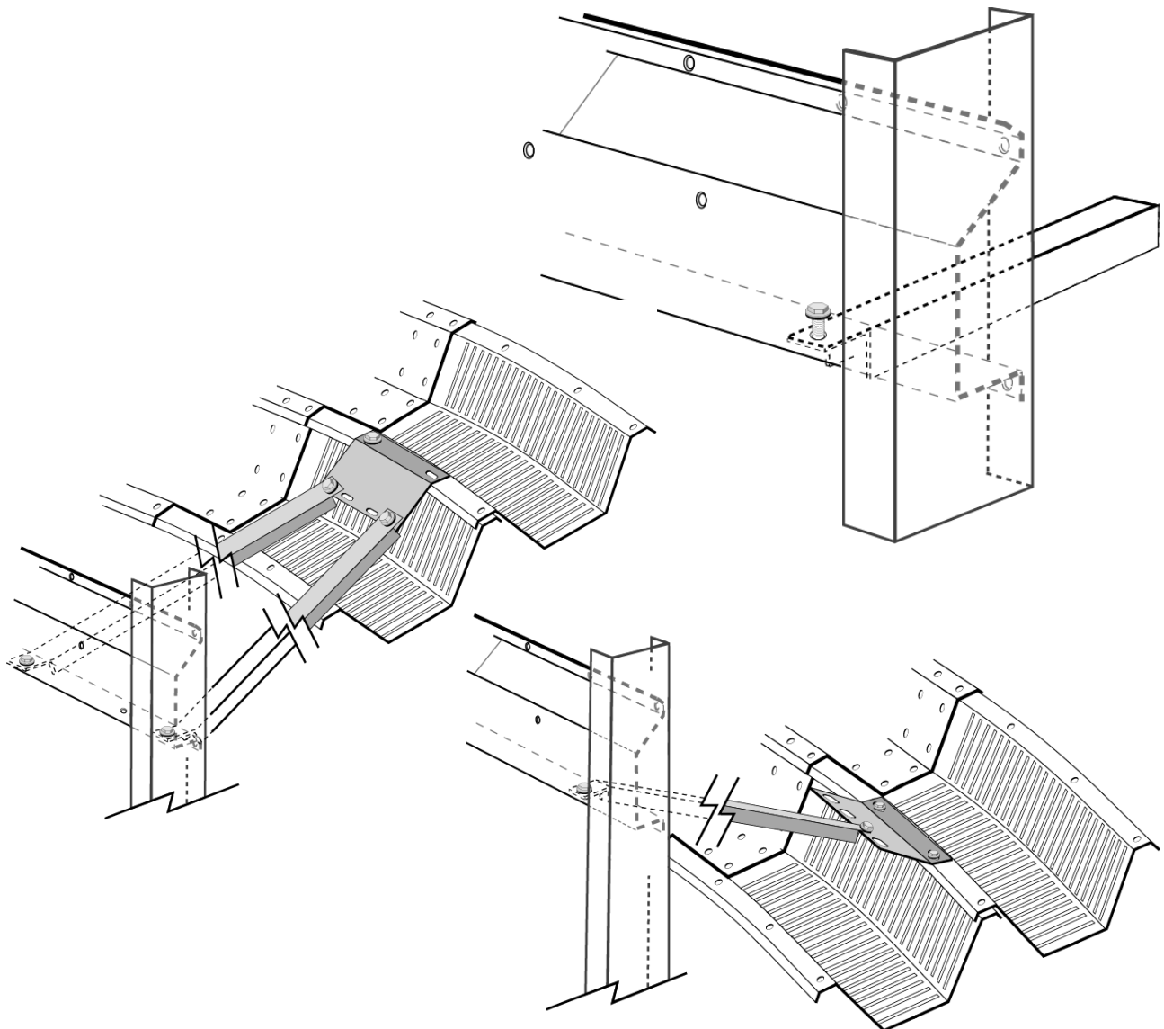
FIGURE 66: SLIDING DOOR WIND BRACING
