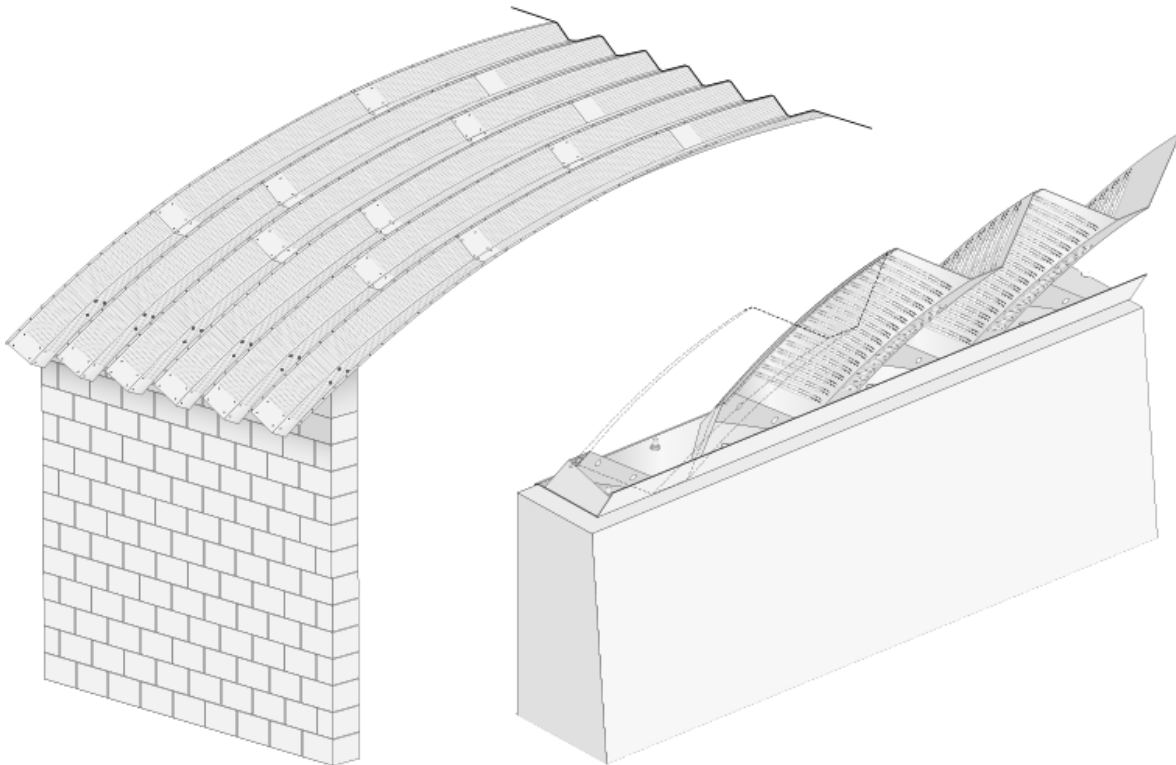
FIGURE 29: ROOF SYSTEM
