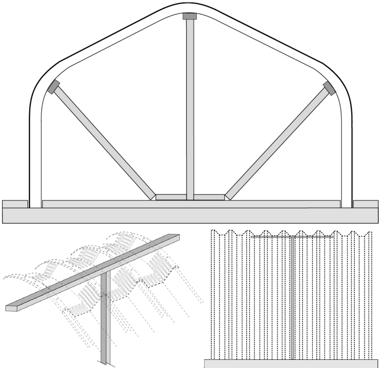
FIGURE 31: TEMPORARY ARCH BRACING
