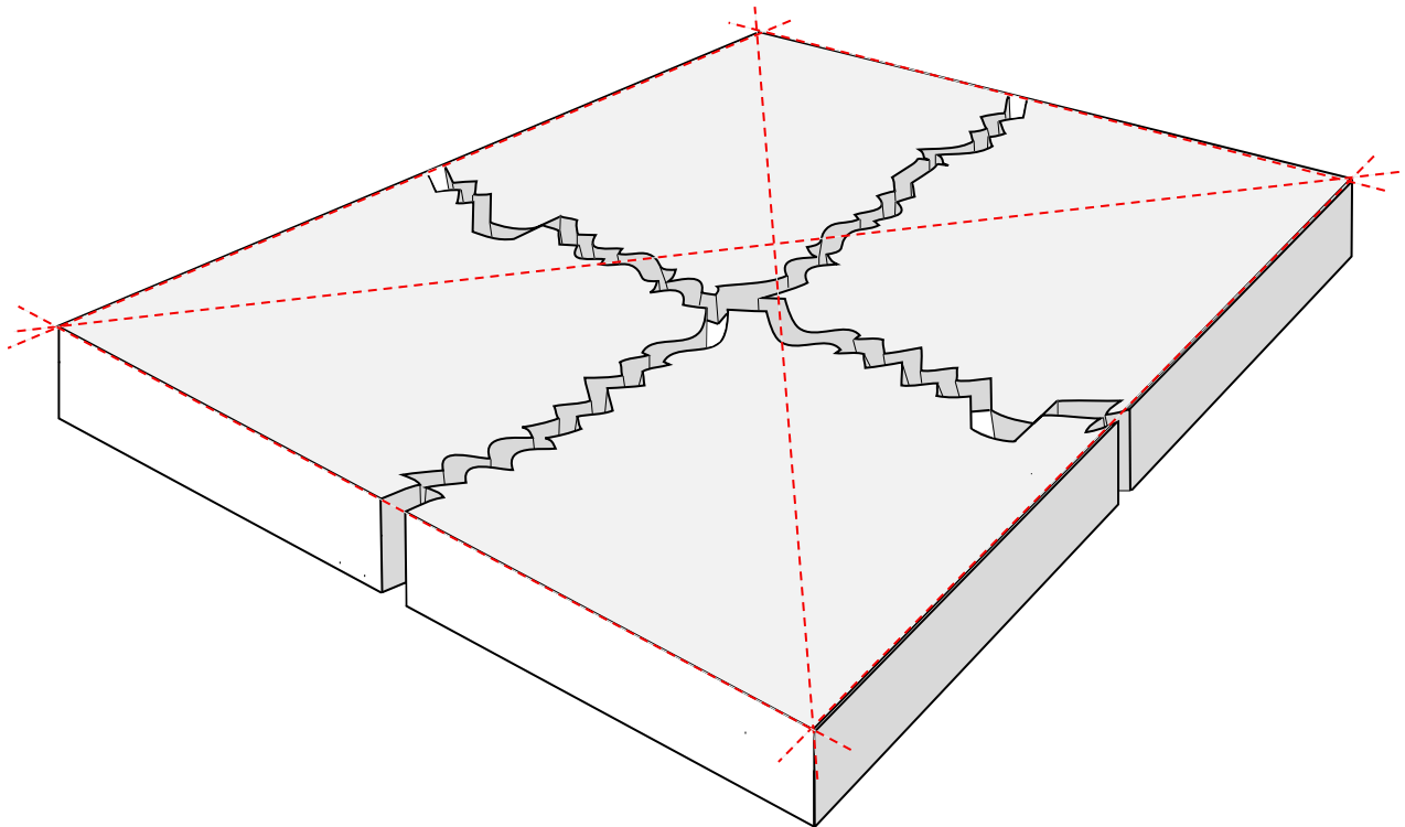
FIGURE 8: MEASURING DIAGONALS
