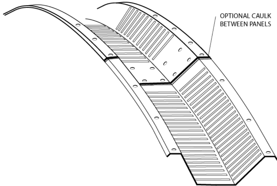
FIGURE 19: OPTIONAL CAULK BETWEEN PANELS
