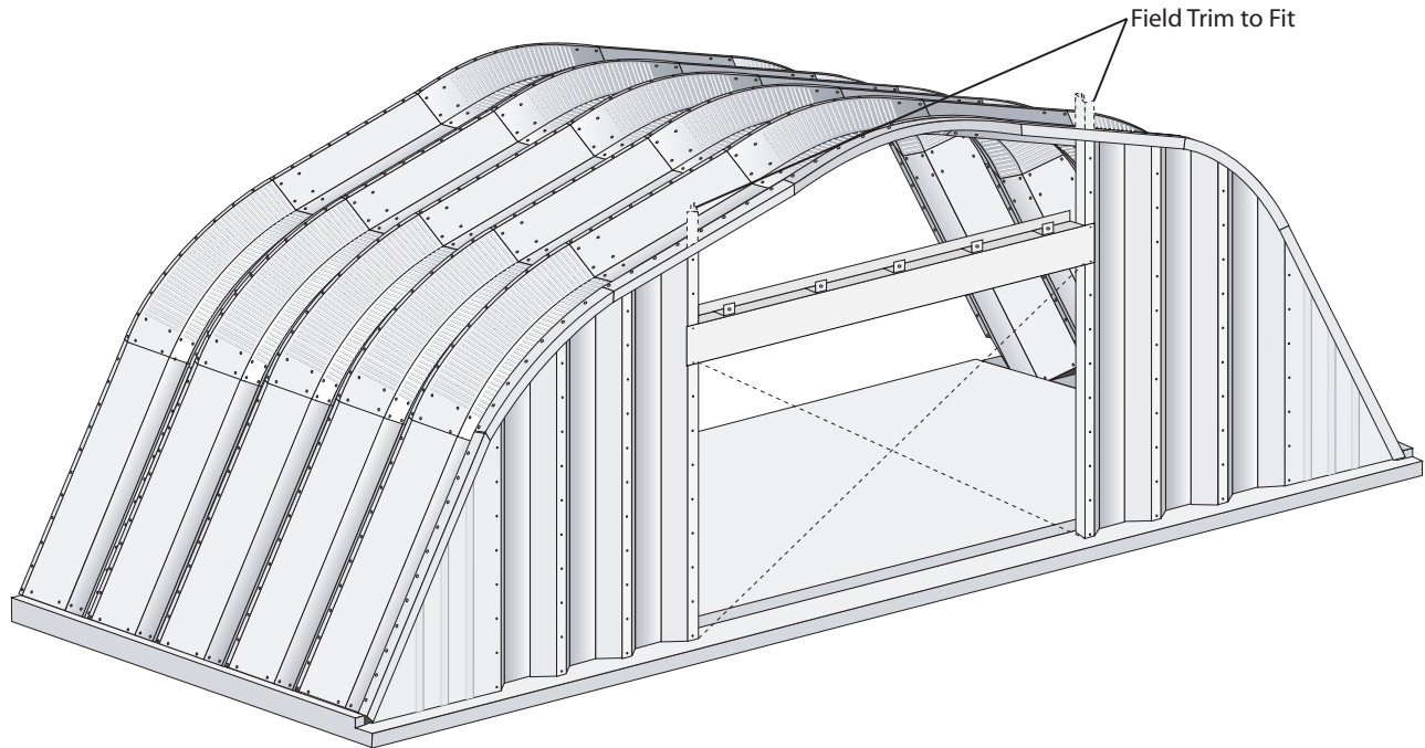
FIGURE 48: INSTALLING DOOR FRAME
