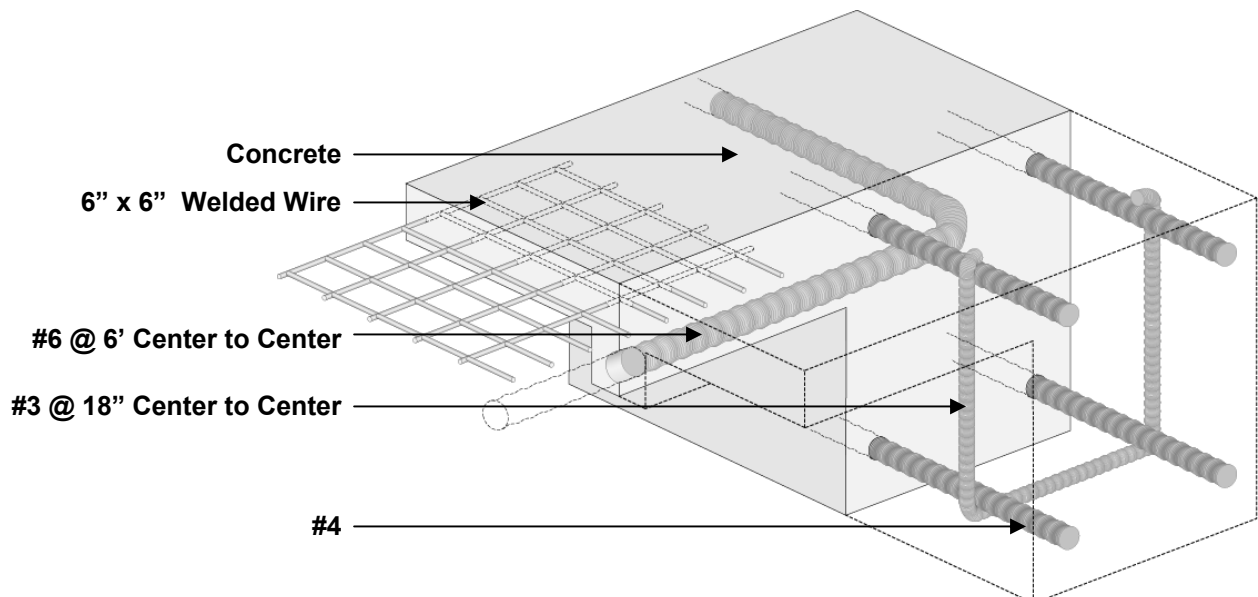
FIGURE 7: CROSS SECTION OF TYPICAL BASE CONNECTOR FOUNDATION
