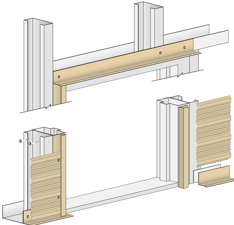
FIGURE 57: FRAMING/FLASHING SERVICE DOORS/WINDOW FRAMES
